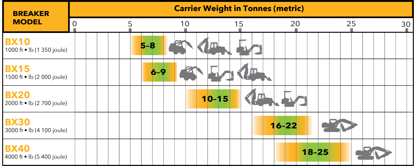
Carrier Sizing Chart
